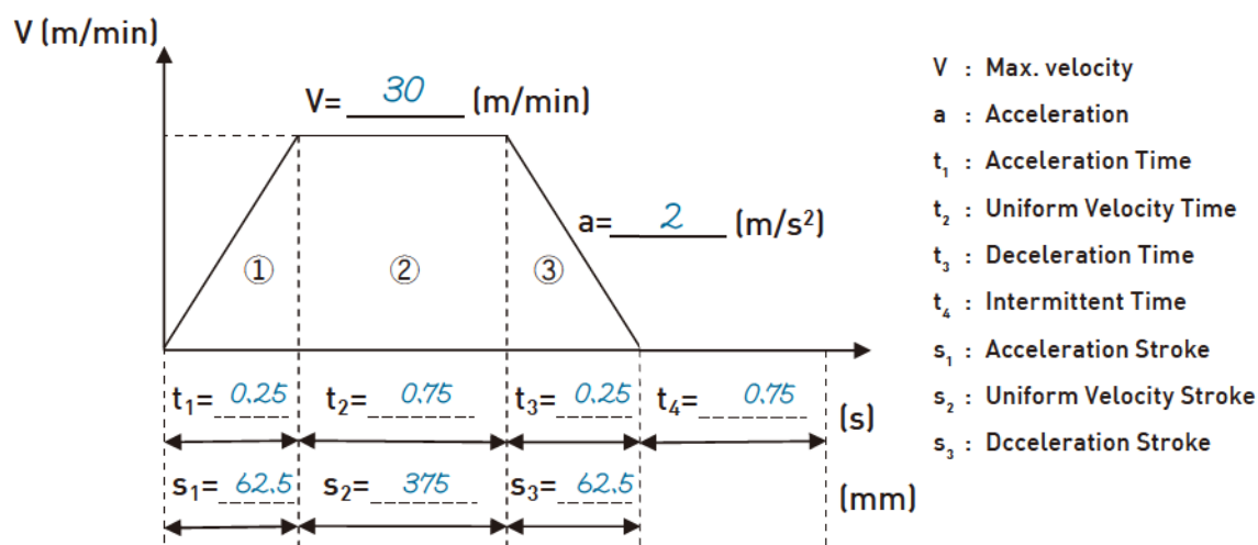
Operation conditions diagram
