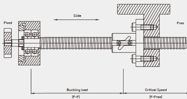
Fig 4.27 Supporting conditions for screw shaft ball nut
