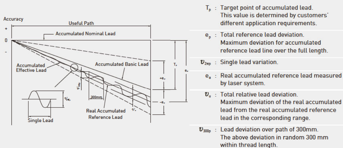
Fig 4.12 HIWIN lead measuring curve of precision ballscrew
