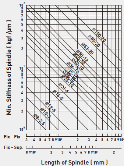
Fig 4.29 Stiffness chart for ballscrew spindle
