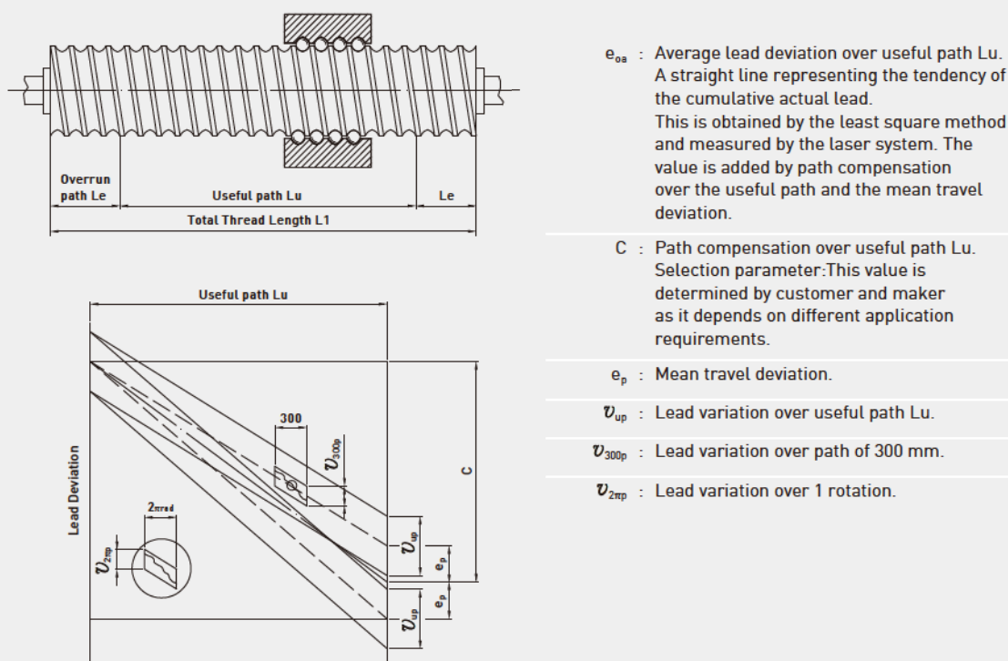
Fig 4.13 DIN lead measuring curve of precision ballscrew
