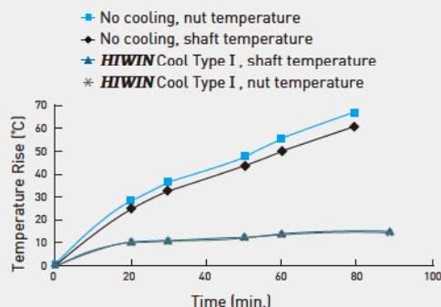
Fig. 8.5 Cool type I : Temperature rise of ballscrew
