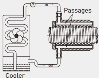
Fig. 8.2 Cool type I with cooler
