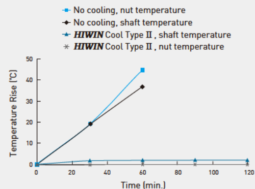
Fig. 8.9 Cool type II : Temperature rise of ballscrew
