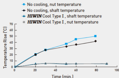
Fig. 8.4 Cool type I : Temperature rise of ballscrew
