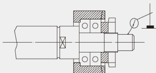
Fig A-3 The Deflection of Ballscrew Spindle
