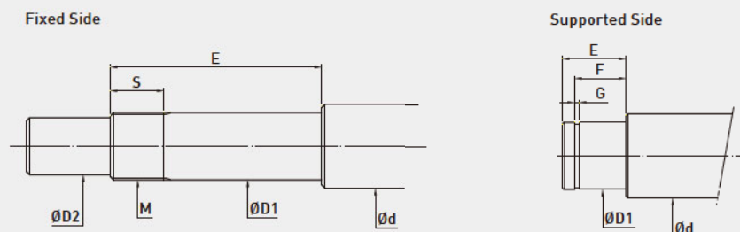
Fig. 3.5 Configurations of spindle ends
