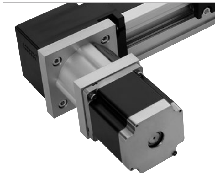
Insert the motor onto the interface flange, attach and tighten the included motor bolts, and tighten the coupling to the motor shaft. Finally, secure the plug over the coupling access window.
