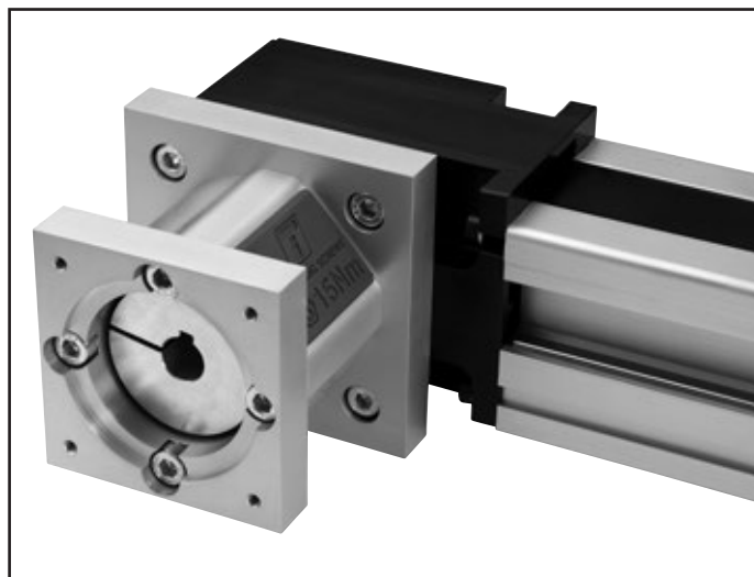
The linear motion system will arrive with the motor interface flange mounted to the unit. In a separate bag, you will find the motor coupling half, the motor bolts and the plug.
